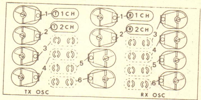
Fig. 9 Trimmer Location Chart
