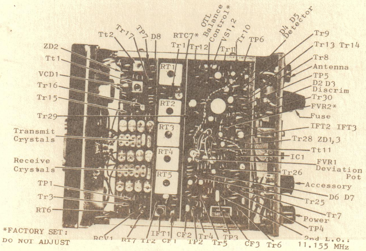
Fig. 7 TOP INSIDE SECTION OF UNIT
