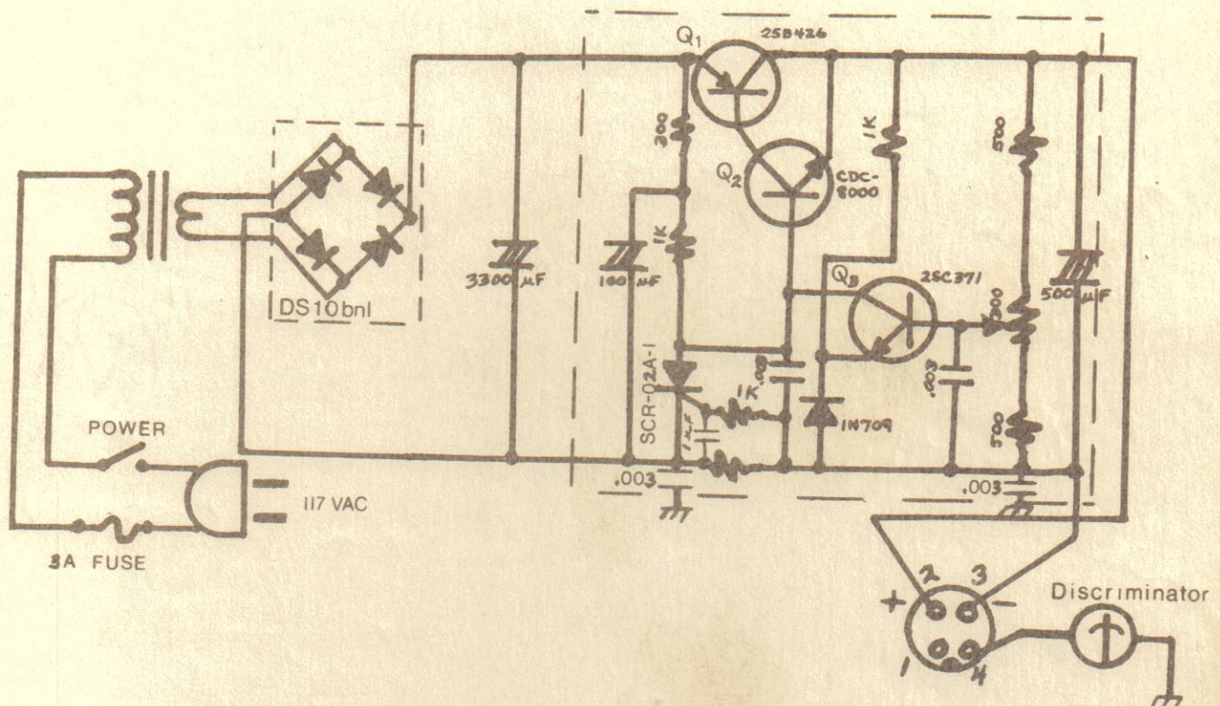
Fig. 11 IC-3P Schematic
