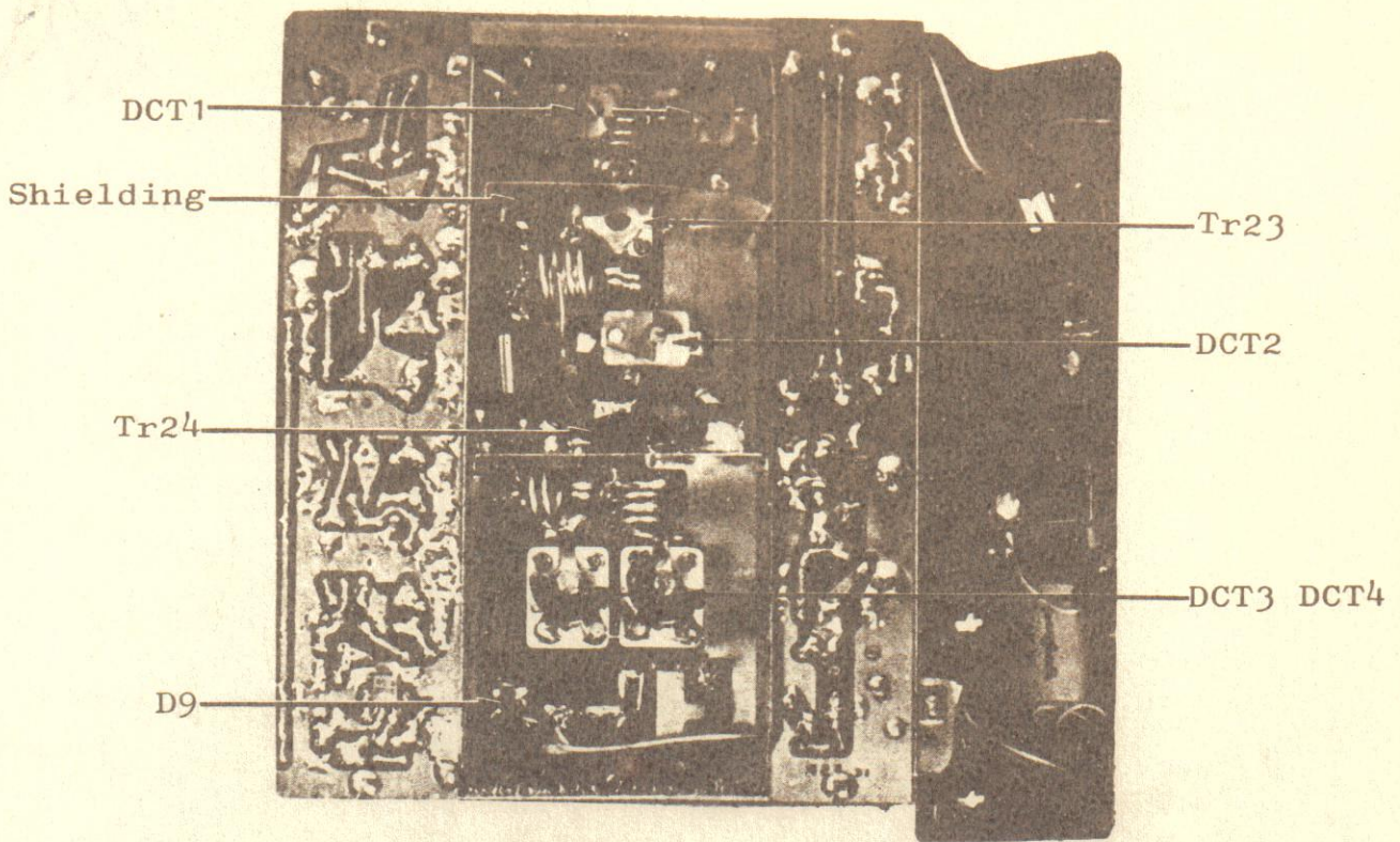
Fig. 8 TRANSMITTER SECTION FOLDED OUT, WITH SHIELD REMOVED Note: Remove section gently from slotted hinge on main chassis.
