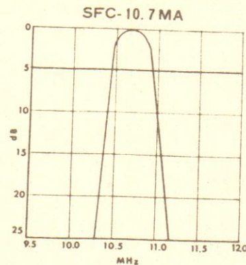
Fig. 2 10.7 MHz Filter Shaping
